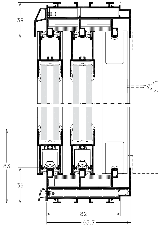
Coupe verticale Vertical cross section Corte vertical
