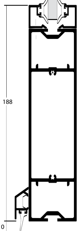
Coupe verticale 2 A B C Vertical cross section Corte vertical
