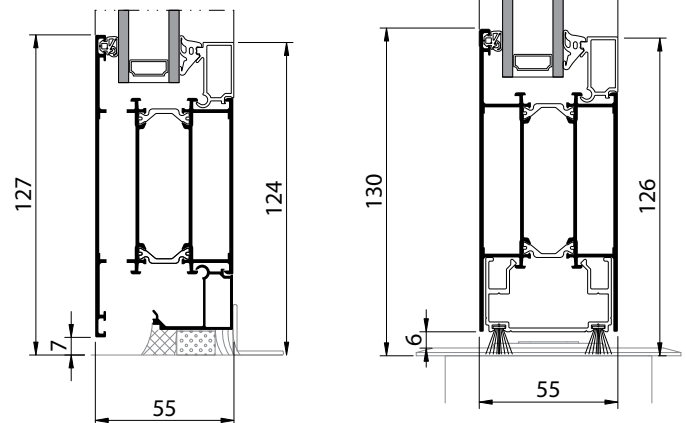
Coupe verticale 1C Vertical cross section Corte vertical
