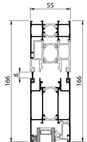
Coupe verticale 1B - B' Vertical cross section Corte vertical
