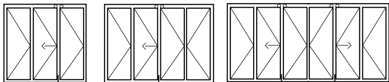
Porte repliable 3,4 et 6 vantaux / 3, 4 & 6-leaf folding door Puerta replegable 3,4 y 6 hojas
