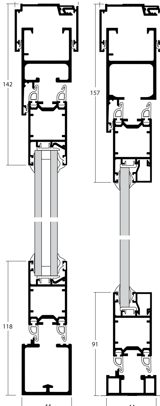
Coupe verticale 1D - D' Vertical cross section Corte vertical
