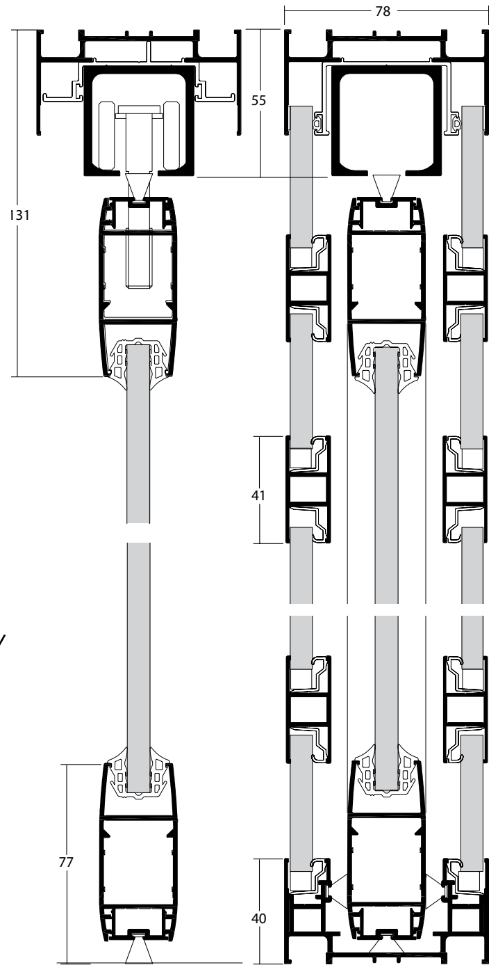
Coupe verticale, 1A, 1A', 1A'' Coupe verticale 1B, 1B', 1B'' Horizontal cross section / Corte horizontal
