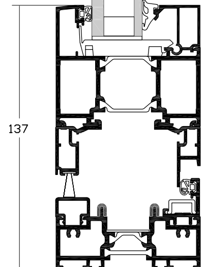
Coupe verticale 1 C – C'
