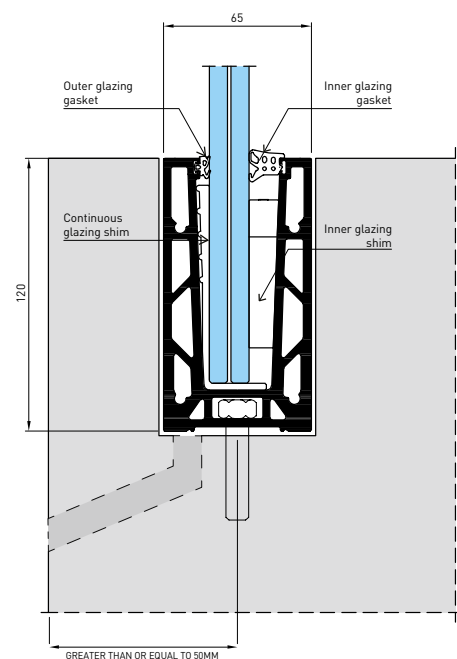
EMBEDDED IN THE SLAB
